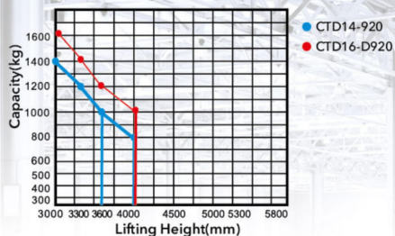
Load Curve
