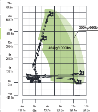
Range of Motion ZT21JE-V (Li)
